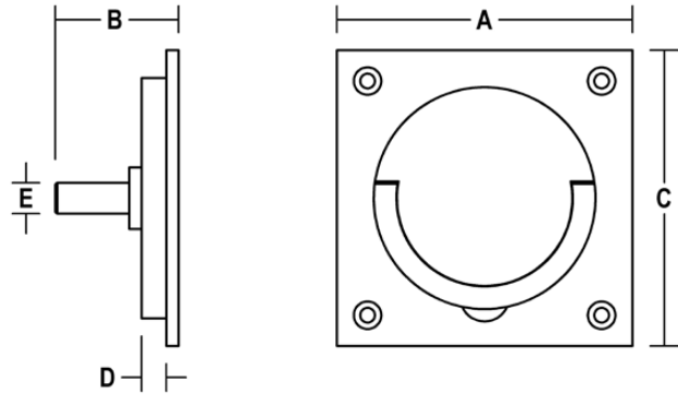
H400 SQUASH COURT RING PULL
