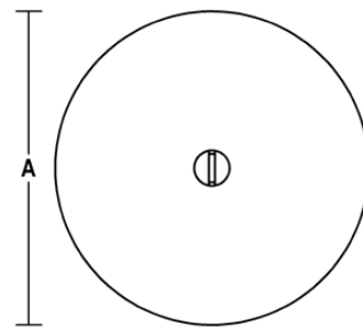
T63 CUT-OUT FILLER PLATE - FOR 2-1/8" HOLE
