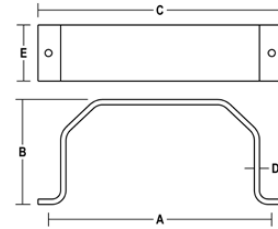
B323 STANDARD DUTY TRIM GUARD - 3.75" PROJ
