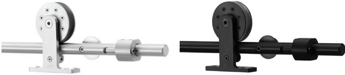
CRT-101-SS & CRT-101-BP Up to 350 lbs. [159 kg] per door
