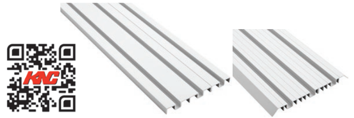
C-202-3 TRIPLE GROOVE GUIDE THRESHOLD 6-3/16" [157.2 mm] wide x 9/16" [14.3 mm] high C-202S-3 TRIPLE GROOVE SLOPED GUIDE THRESHOLD 7-15/32" [189.4 mm] wide x 9/16" [14.3 mm] high
