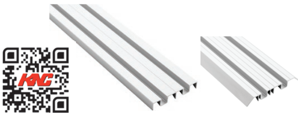
C-238 DOUBLE GROOVE GUIDE THRESHOLD 3-1/2" [88.9 mm] wide x 9/16" [14.3 mm] high C-238S DOUBLE GROOVE SLOPED GUIDE THRESHOLD 4-19/32" [116.4 mm] wide x 9/16" [14.3 mm] high
