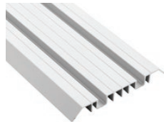
C-202 DOUBLE GROOVE GUIDE THRESHOLD 4-1/4" [108 mm] wide x 9/16" [14.3 mm] high C-202S DOUBLE GROOVE SLOPED GUIDE THRESHOLD 5-11/32" [135.4 mm] wide x 9/16" [14.3 mm] high
