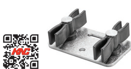
C200D-138 BYPASS GUIDE 1-1/2" [38.1 mm] wide x 13/16" [20.6 mm] high Center to Center of guides 1-3/4" [44.5 mm]
